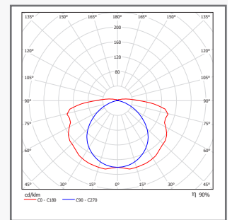
Polar curve
