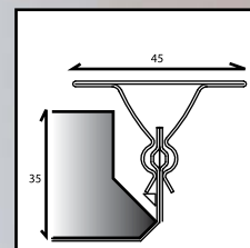
Burgess "Spring Tee" or Orcal Spring Tee
