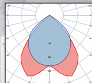
cd/klm \eta = 55\% — C0 - C180 — C90 - C270
