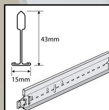
Flat Table 15mm Tee 43mm high
