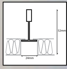
TruGrid T24 system
