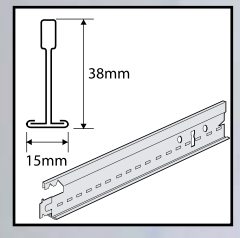
Flat Table 15mm Tee 38mm or 43mm high
