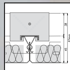
System 120 Long Span Spring Tee
